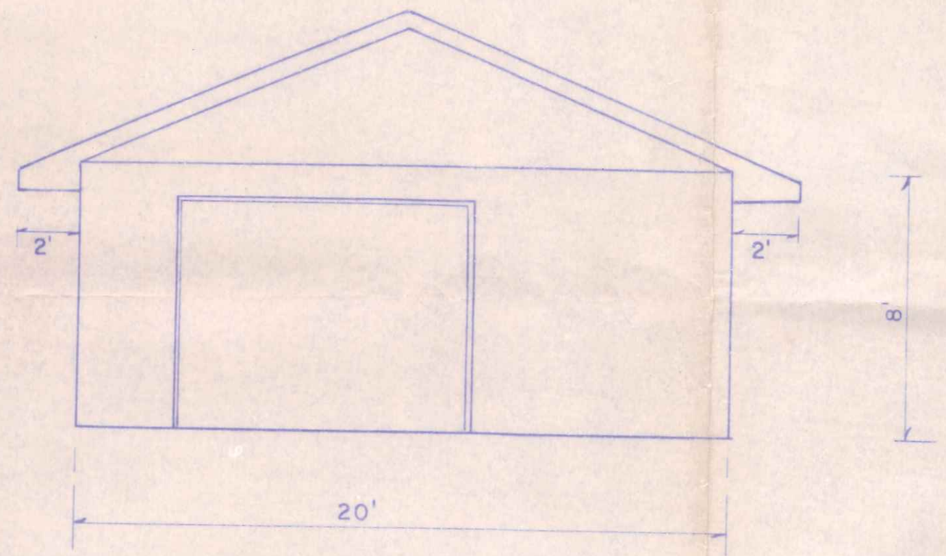
WEST ELEVATION Scale 1/4" = 1'-0"
