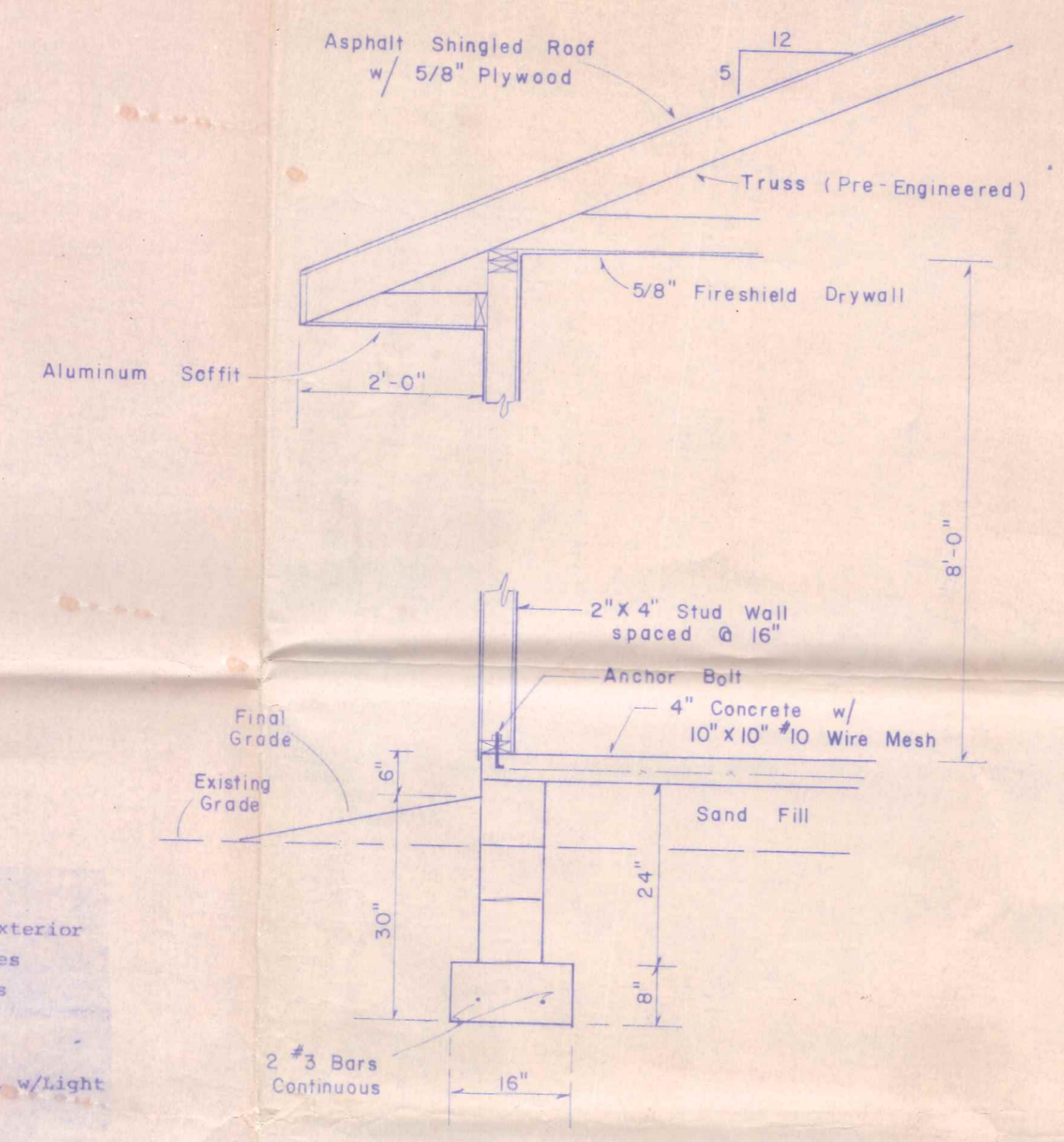
WALL & FOOTER SECTION Scale 3/4" = 1'-0"
